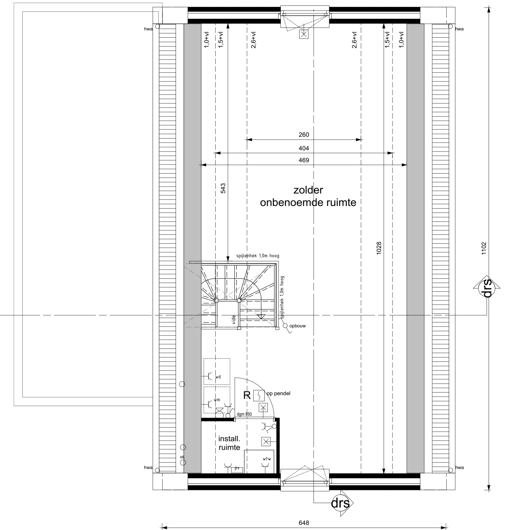
Zolder
